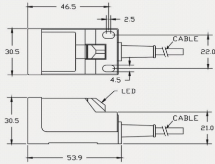
Pre-wired 2M Cable ABS
